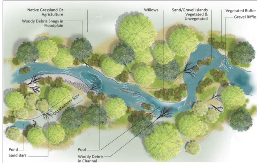
Figure 3. Restored Channel Prototype – Plains Segments.
