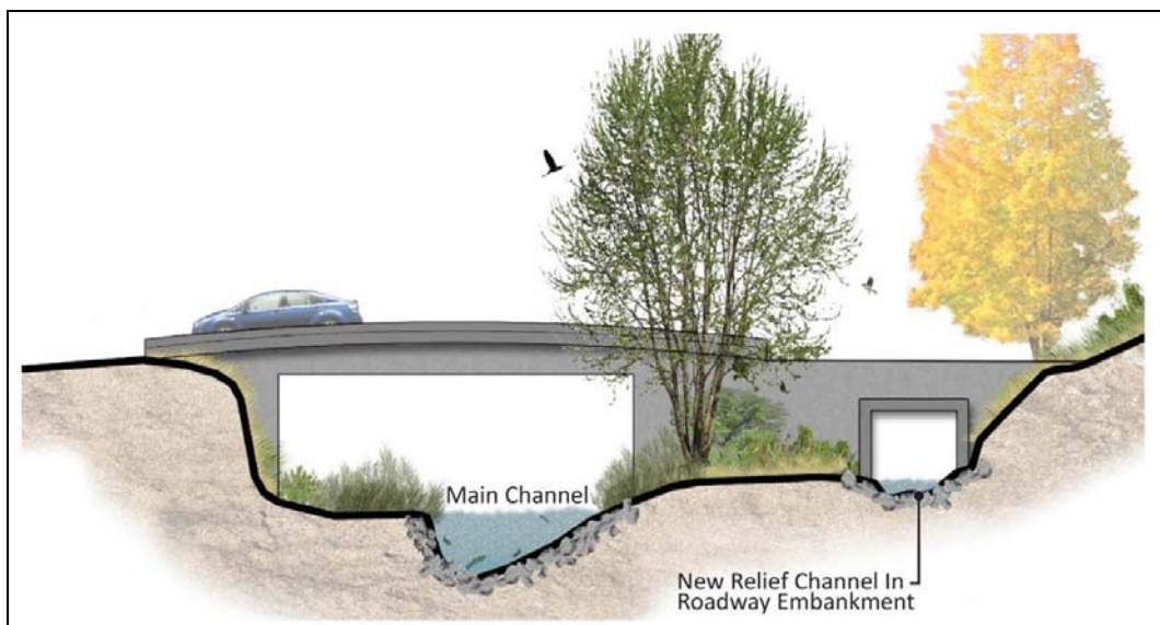
Figure 5.17. Relief structure in roadway embankment.
